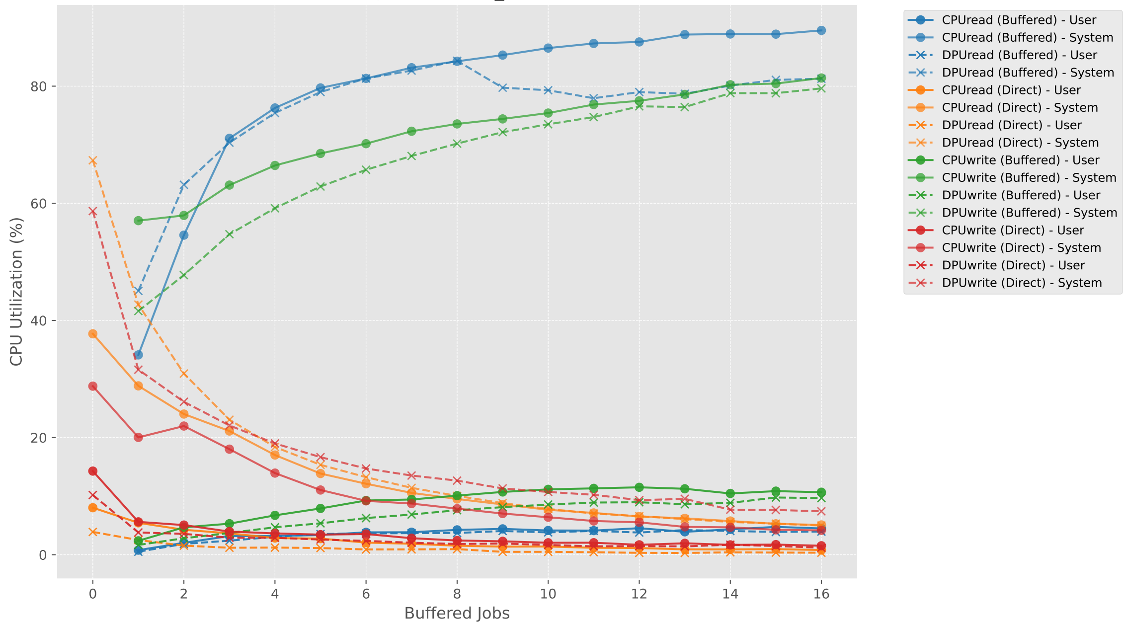
CPU Utilization vs Buffered Jobs (direct1_bufferedN) - SEQ (CPU vs DPU)
